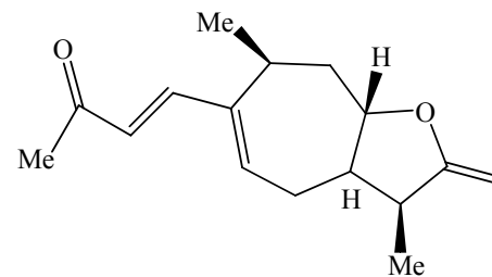
11α-13-dihydroxy xanthatin
