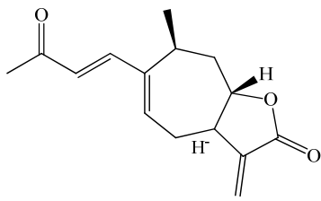
(-)-xanthatin
