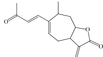
deacetyl xanthumin
