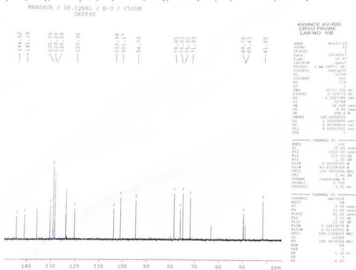
Figure 2 - ^{13}\text{C} NMR spectrum of lateroside
