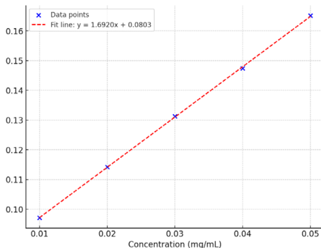
Figure 4. Calibration curve of the ascorbic acid
