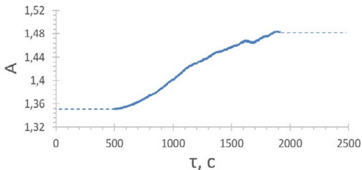
Figure 5. Kinetic dependence of the change in the absorption minimum of Mo-V blue (502 nm) with KNO 3
