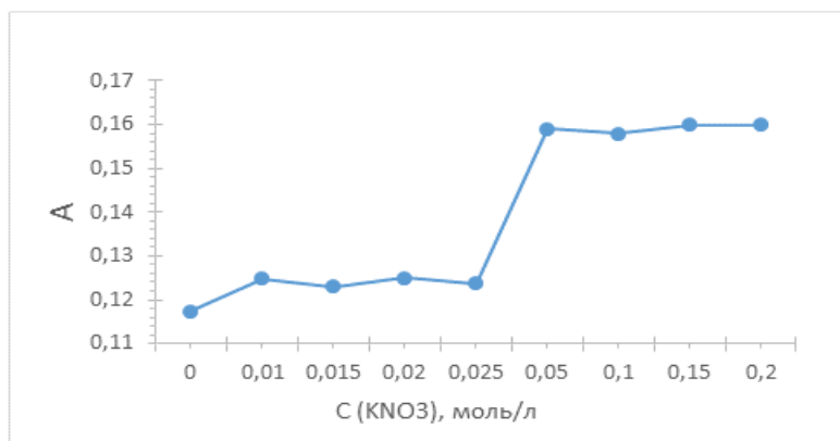
Figure 8. Dependence of optical density on Mo-V blue in the region of minimum absorption (502 nm) of fire concentration electrolyte ( \text{KNO}_3 )
