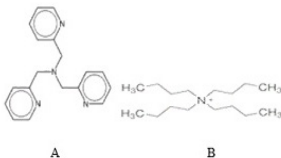
Figure 1. Ligands: A - Tris - (2-pyridylmethyl)amine (tpma); B - Tetrabutylammonium cyanide
