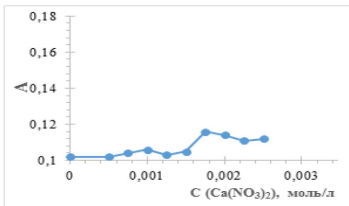
Figure 2. Dependence of the change in optical density (502 nm) on the concentration of electrolyte \text{Ca}(\text{NO}_3)_2
