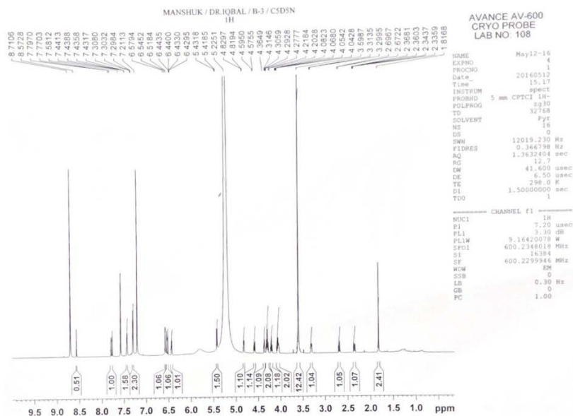
Figure 1 - ^1\text{H} NMR spectrum of lateroside
